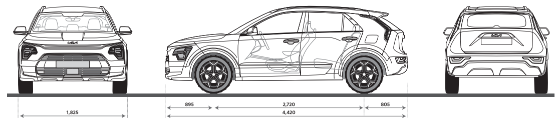
Dimensions Niro Hybride et Hybride Rechargeable (mm)
